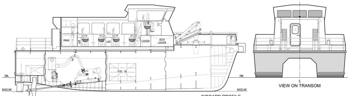
INBOARD PROFILE
