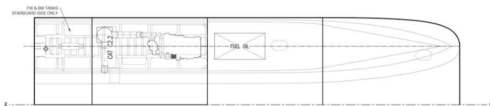
HALF PLAN VIEW ON HULL
