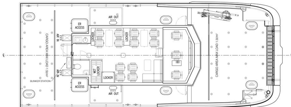
PLAN VIEW ON MAIN DECK
