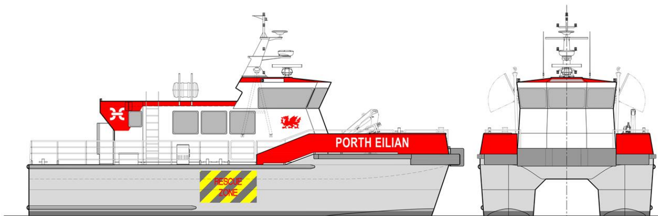
OUTBOARD PROFILE
