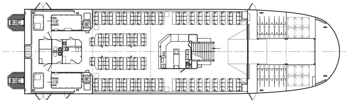
Lower Deck Plan
