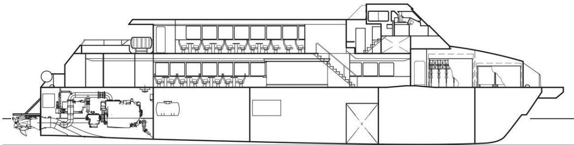
Inboard Profile
