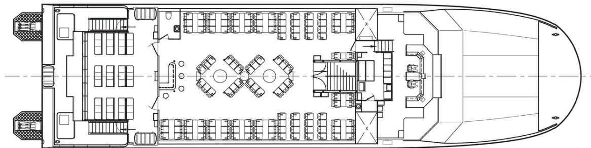
Upper Deck Plan
