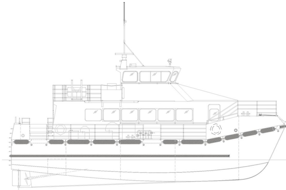
Outboard Profile
