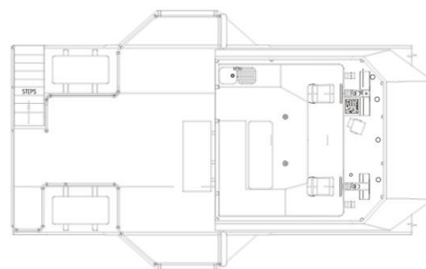
Bridge Deck Plan
