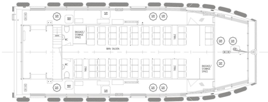
Passenger Deck Plan
