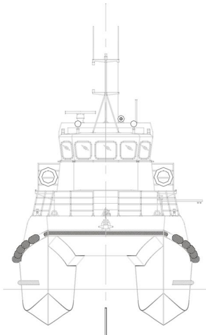
Bow View
