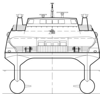
Bow View
