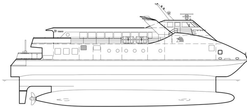
Outboard Profile
