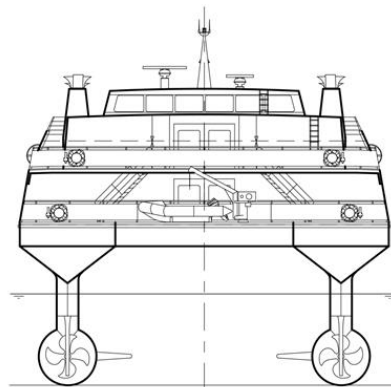
Stern View
