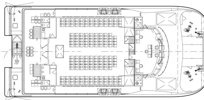
Passenger Deck Plan
