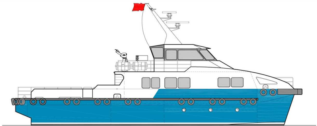
OUTBOARD PROFILE
