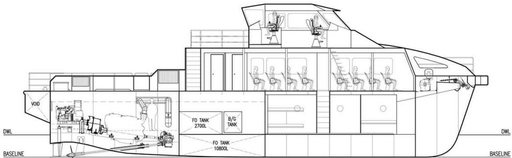
INBOARD PROFILE
