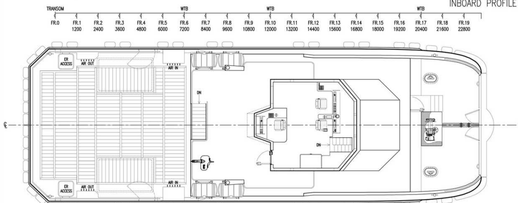
PLAN VIEW BRIDGE
