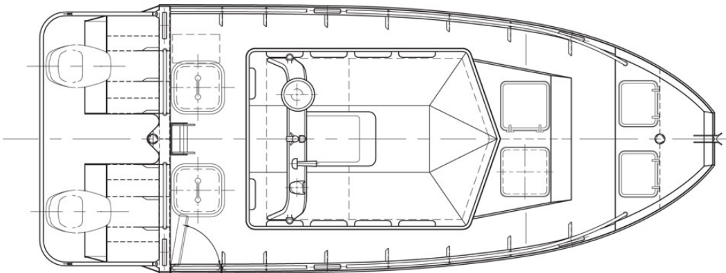
Plan on Wheelhouse
