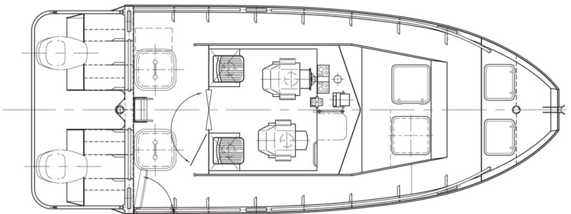
Plan on Main Deck
