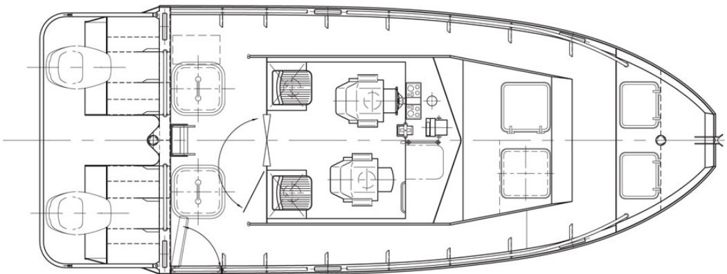
Plan on Main Deck
