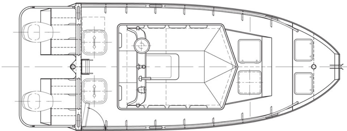
Plan on Wheelhouse
