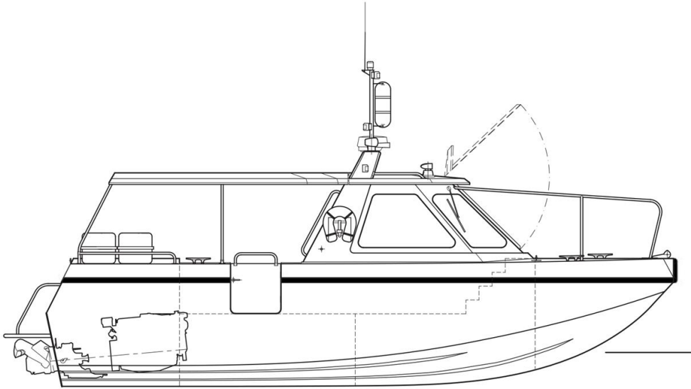
Outboard Profile
