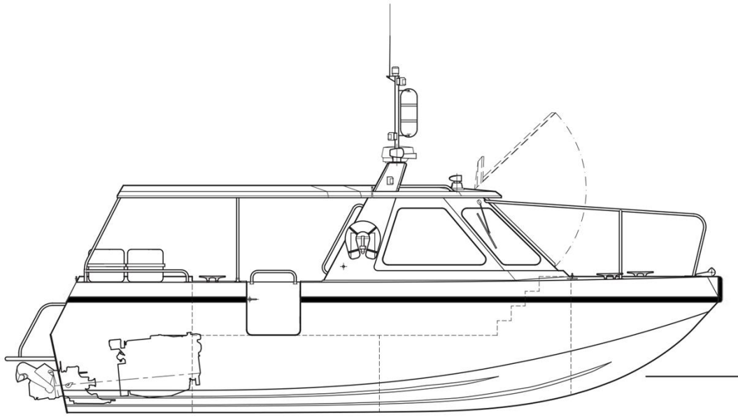
Outboard Profile
