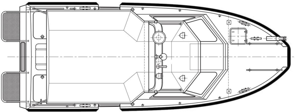
Deck View
