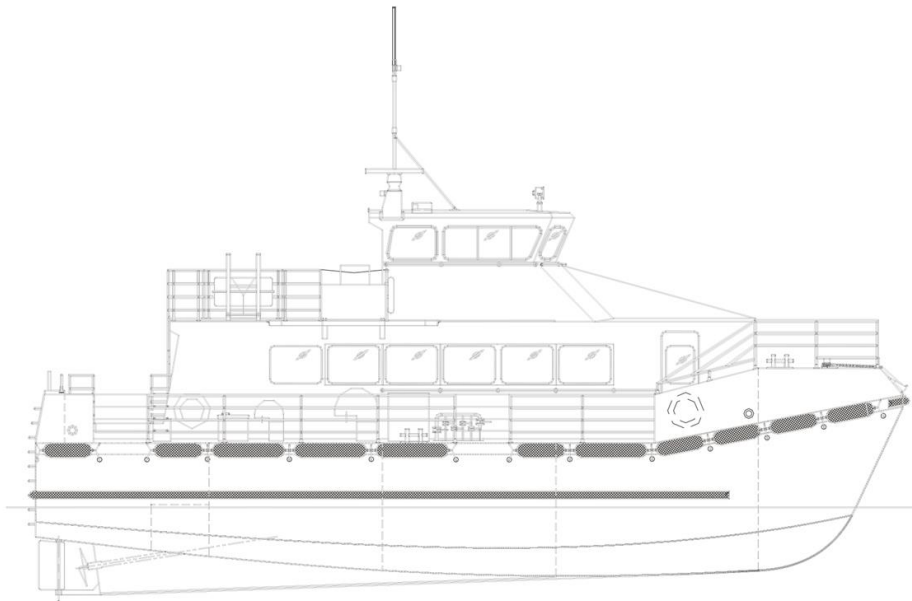
Outboard Profile
