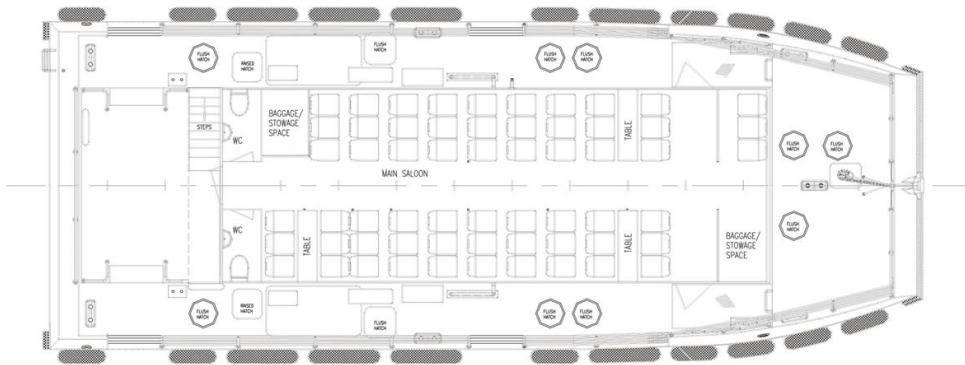
Passenger Deck Plan
