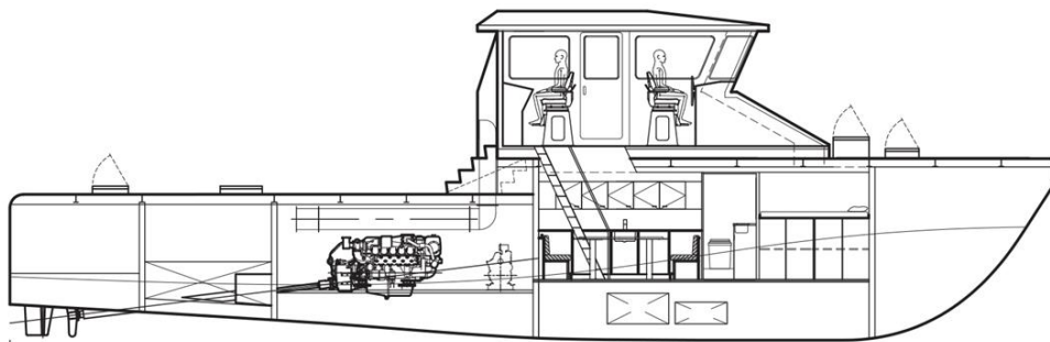
Inboard Profile
