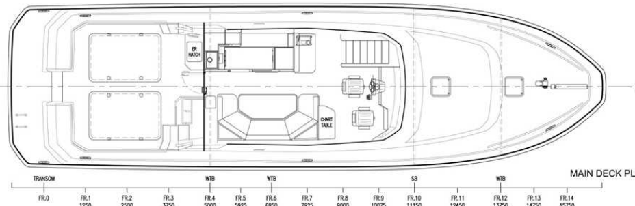
EXTERIOR DECK PLAN
