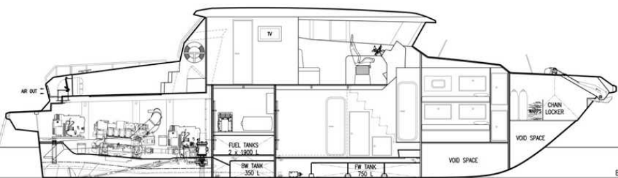
INBOARD PROFILE
