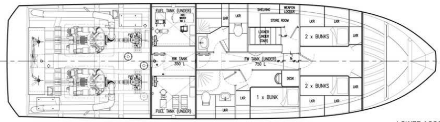
LOWER ACCOM. PLAN
