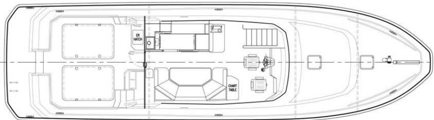
MAIN DECK PLAN
