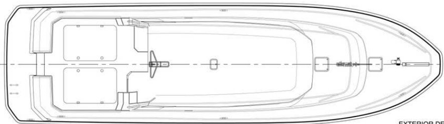
EXTERIOR DECK PLAN
