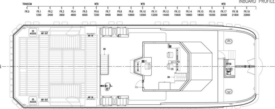
PLAN VIEW BRIDGE
