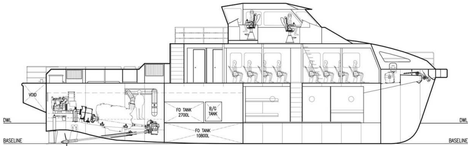
INBOARD PROFILE
