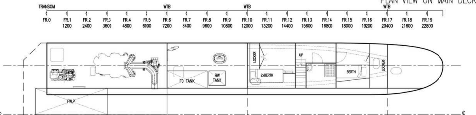
PLAN VIEW ON MAIN DECK
