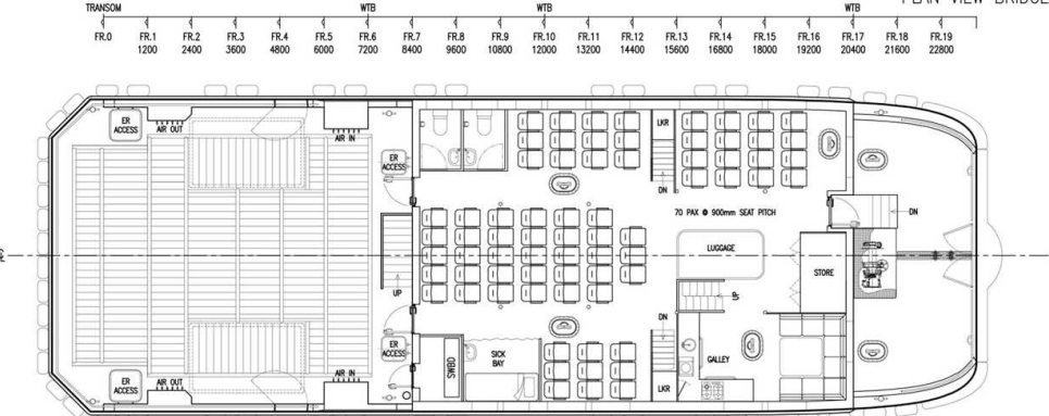
PLAN VIEW ON MAIN DECK
