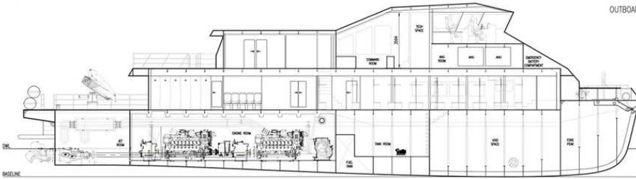
INBOARD PROFILE
