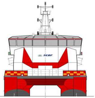
VIEW ON BOW
