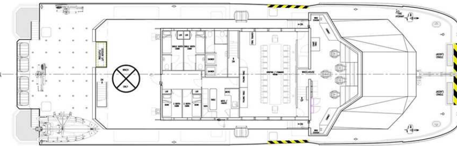
PLAN VIEW UPPER DECK
