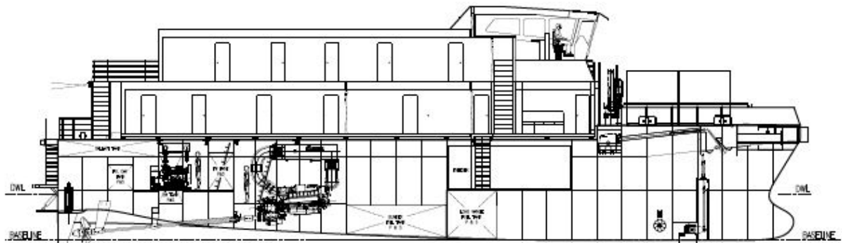
INBOARD PROFILE
