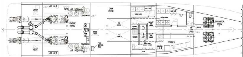
PLAN VIEW ON HULL
