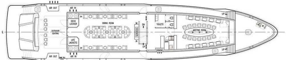
PLAN VIEW ON MAIN DECK
