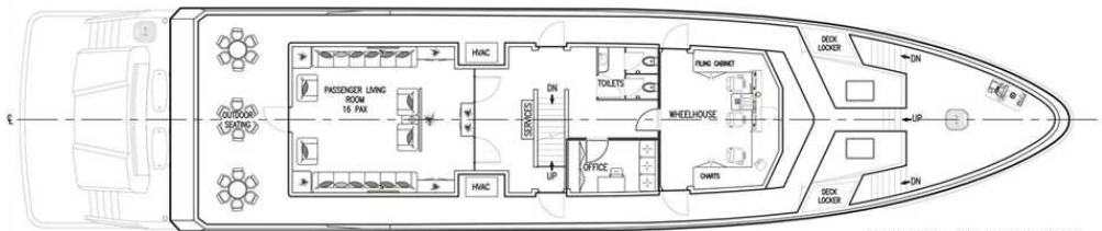
PLAN VIEW ON UPPER DECK
