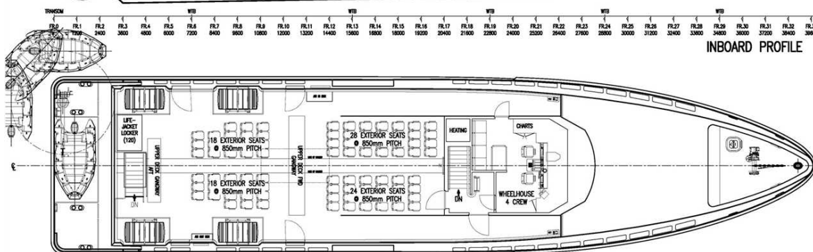
PLAN VIEW ON UPPER DECK
