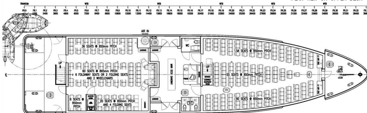
PLAN VIEW ON MAIN DECK
