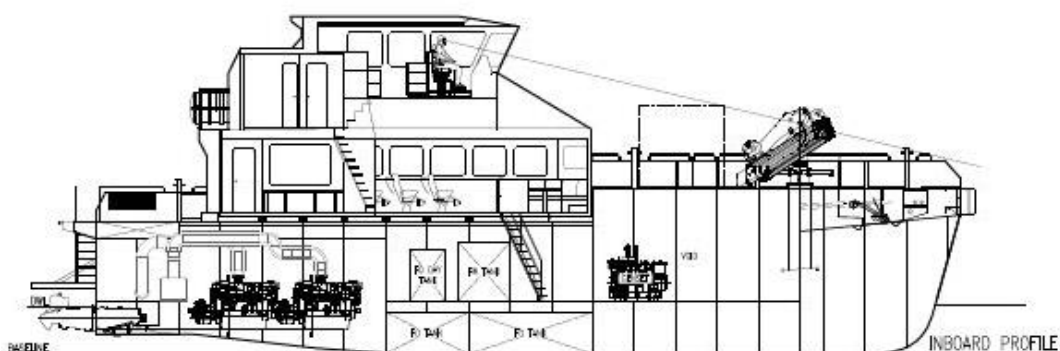
INBOARD PROFILE
