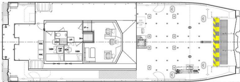
PLAN VIEW BRIDGE DECK
