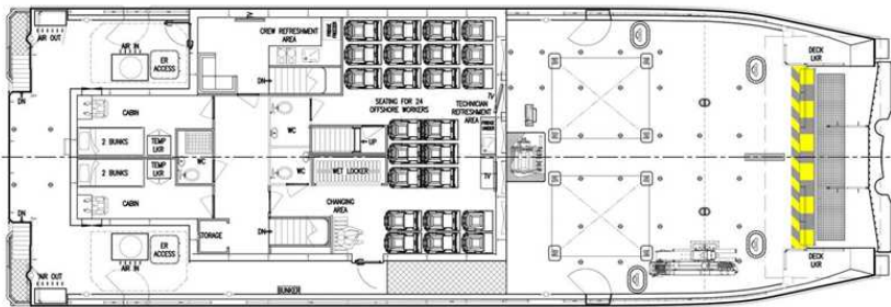
PLAN VIEW MAIN DECK
