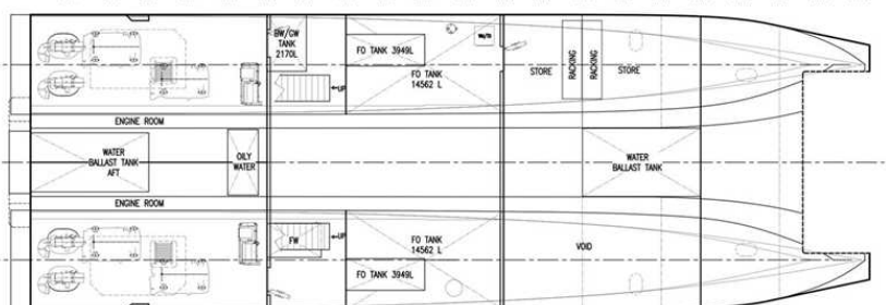
PLAN VIEW ON HULL
